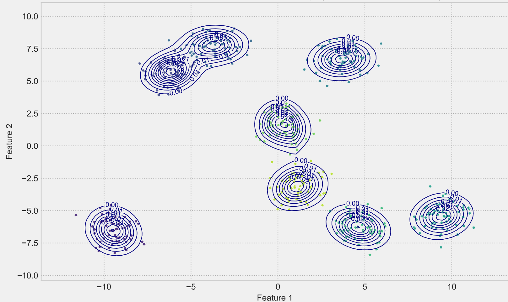
DPM Posterior Predictive Density (Multi-Chain Robust)
